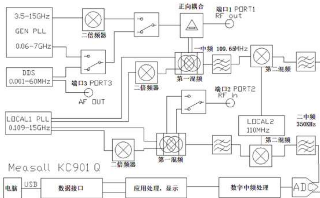
Chart 6-1: KC901Q's Schematic Diagram
