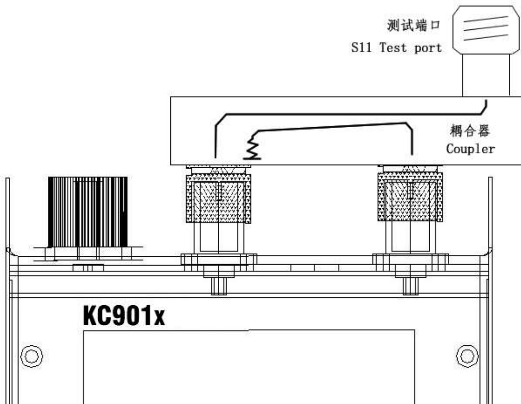
Chart 3-2: Connect the coupler
