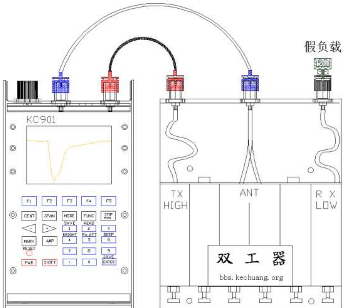
Chart 4-1: Example for connection method of duplexer measurement
