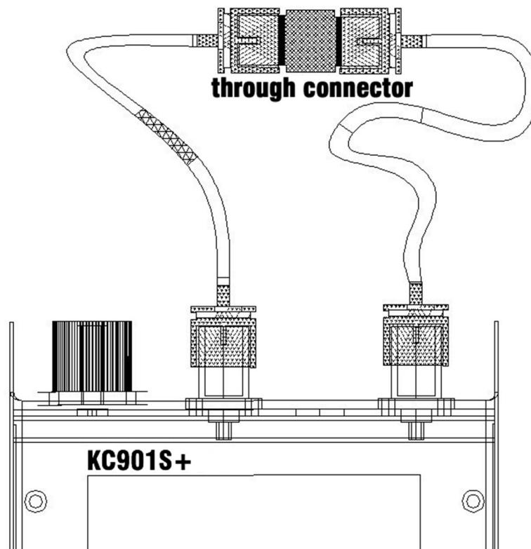
Chart 3-1B: Connect two cables in calibration
