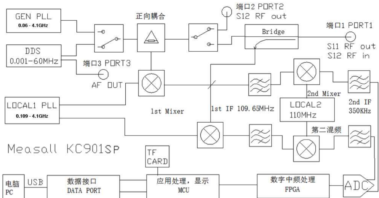
Chart 6-1: KC901S+'s Schematic Diagram
